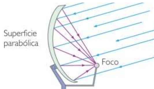
Fig 8 Antena Offset.
