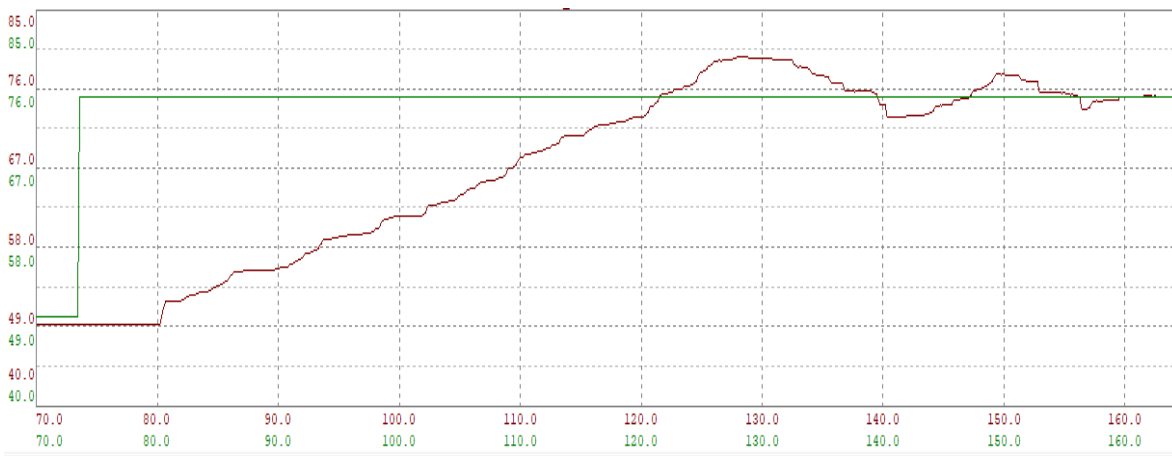
Fig. 7.6 Setpoint 75%
